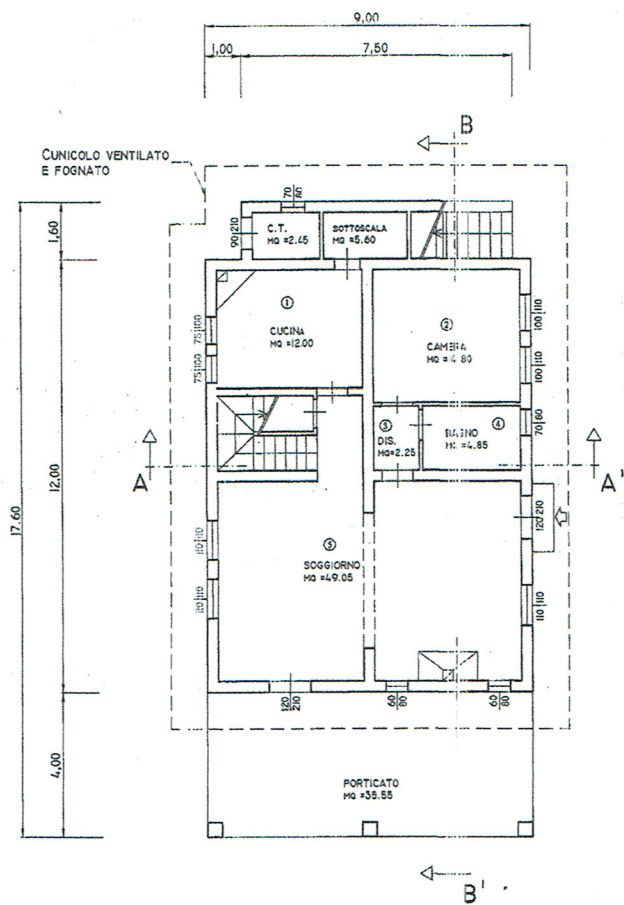
PIANO TERRA
